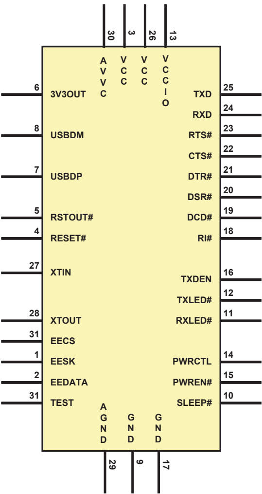
Figure 2 Pin-Out (Schematic Symbol )
