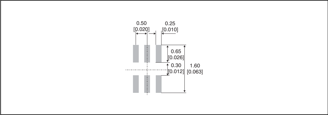
Figure 23. \mu QFN 6 leads footprint dimensions in mm [inches]
