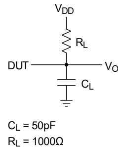
Figure 7. Tri-State Low Load Circuit
