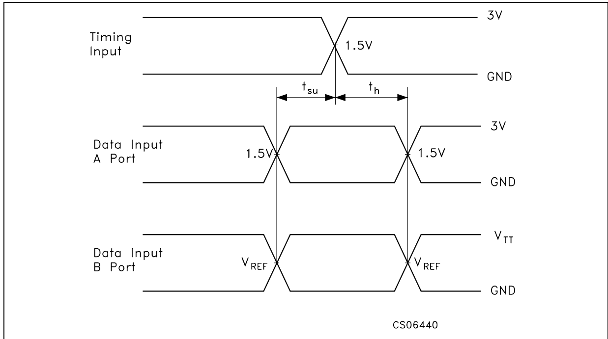
WAVEFORM 4: SETUP AND HOLD TIME
