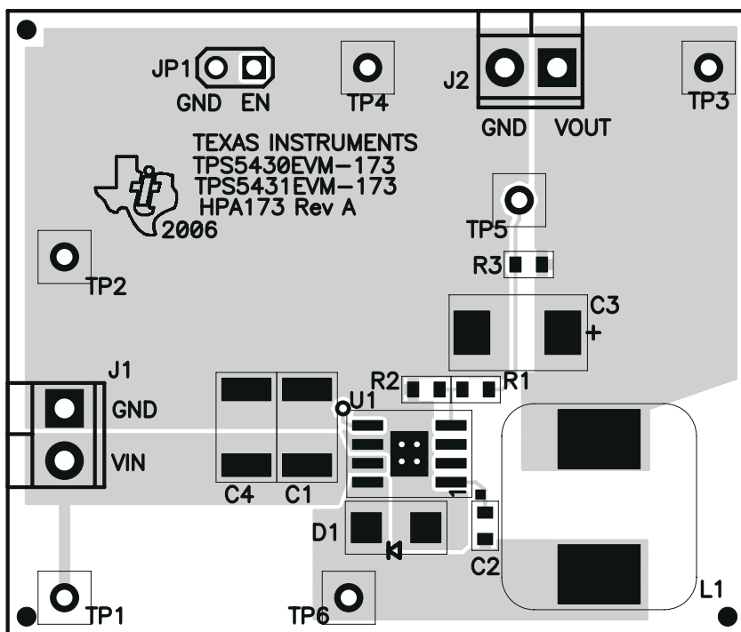
Figure 3-3. Top-Side Assembly
