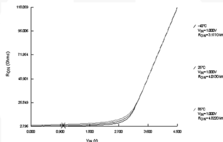
Figure 9. R_{ON} Switch On Resistance, I_{ON}=13mA
