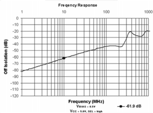
Figure 7. Off Isolation
