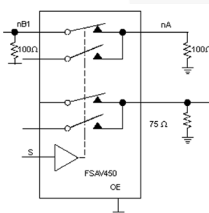
Figure 14. Crosstalk
