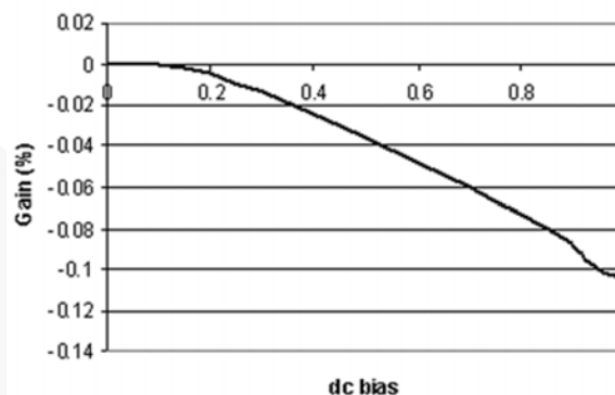
Figure 5. Differential Gain vs. DC bias
