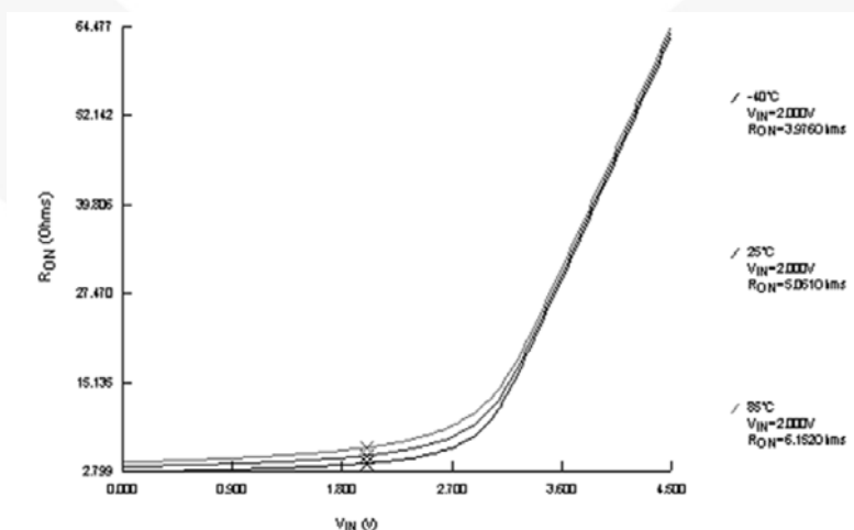
Figure 10. R_{ON} Switch On Resistance, I_{ON}=26mA
