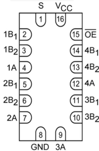
Figure 3. DQFN Pin Assignments
