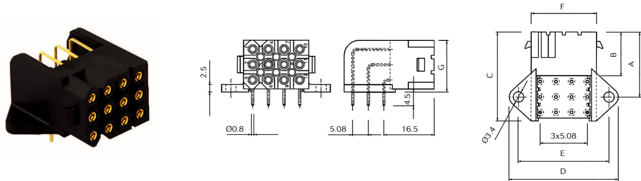
Right angle boardmount receptacle delivered with female PCB contacts (SMS GE53)
