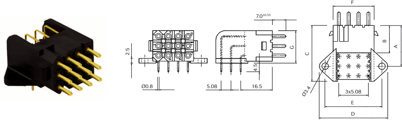
Right angle boardmount receptacle delivered with male PCB contacts (SMS GE63)
