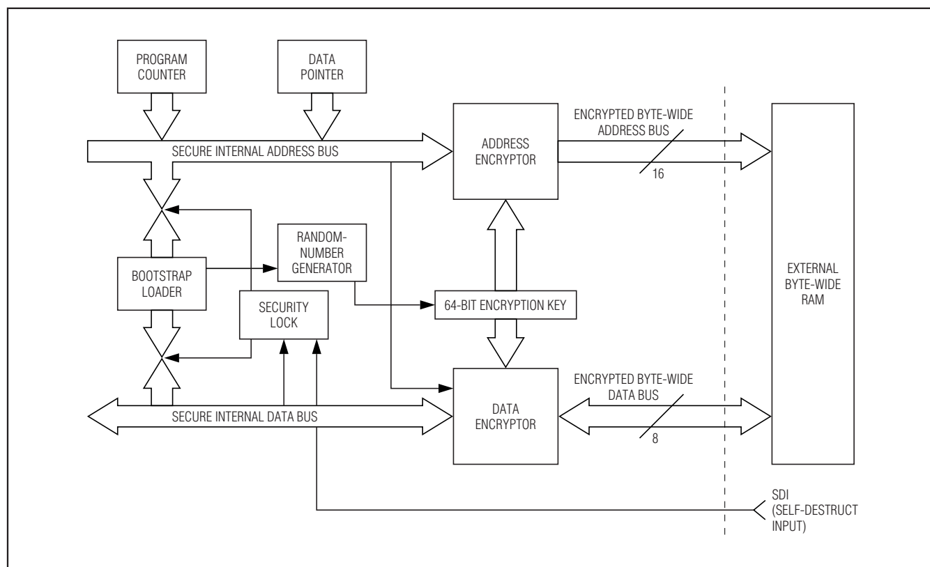
Figure 9. Security Circuitry
