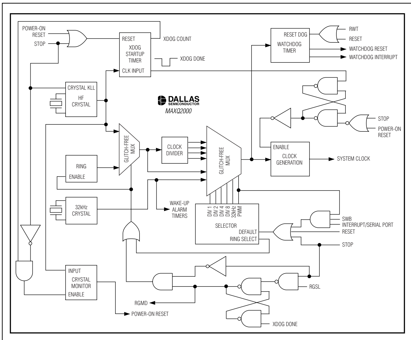
Figure 2. Clock Sources
