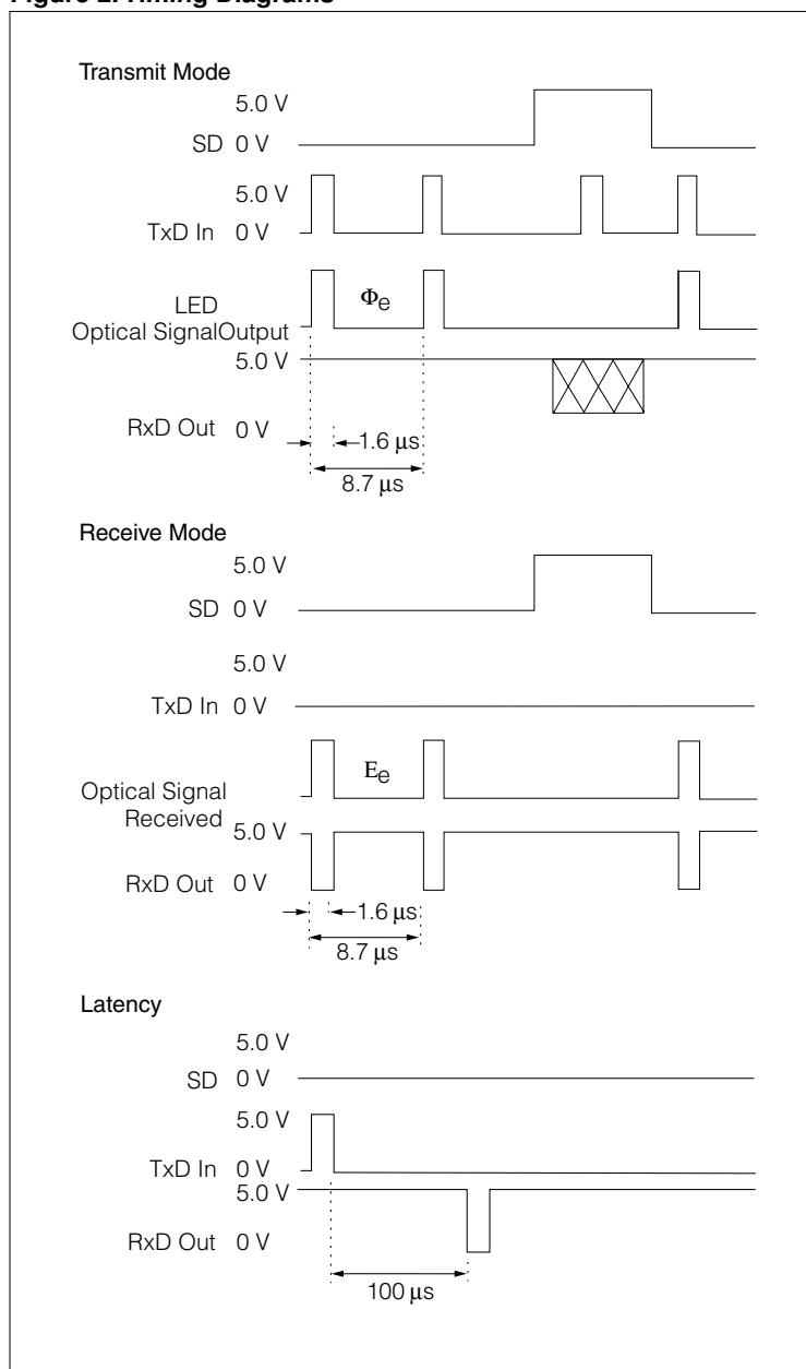
Figure 2. Timing Diagrams
