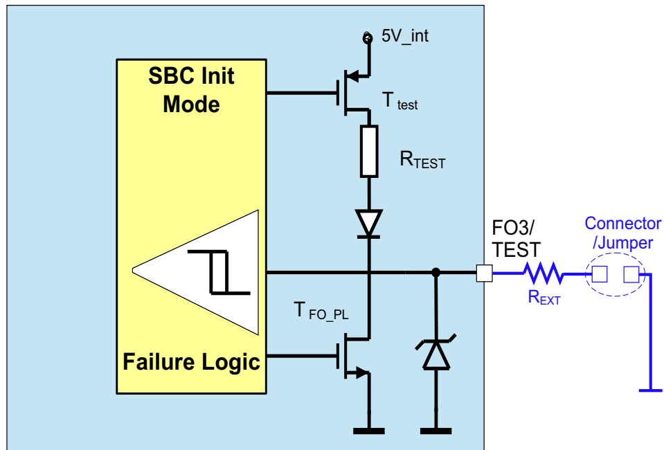
Figure 55 Hint for Increasing the Robustness of pin FO3/TEST during Debugging or Programming
