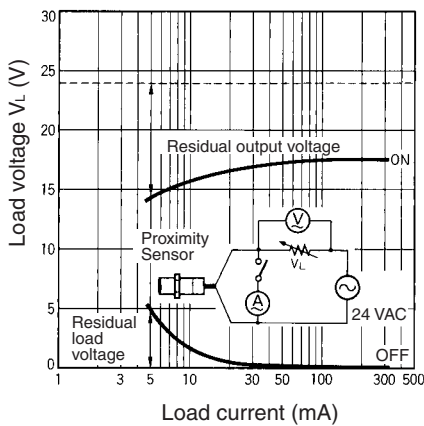
24 VAC
