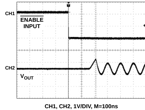
FIGURE 26. ENABLED RESPONSES
