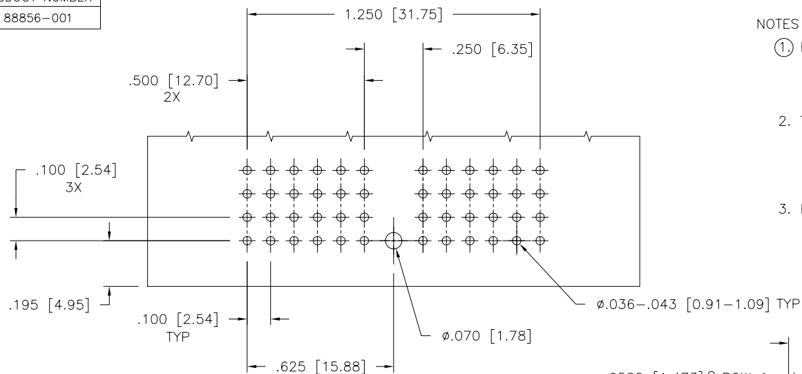
RECOMMENDED PCB LAYOUT FOR 2 MODULE RECEPTACLE
