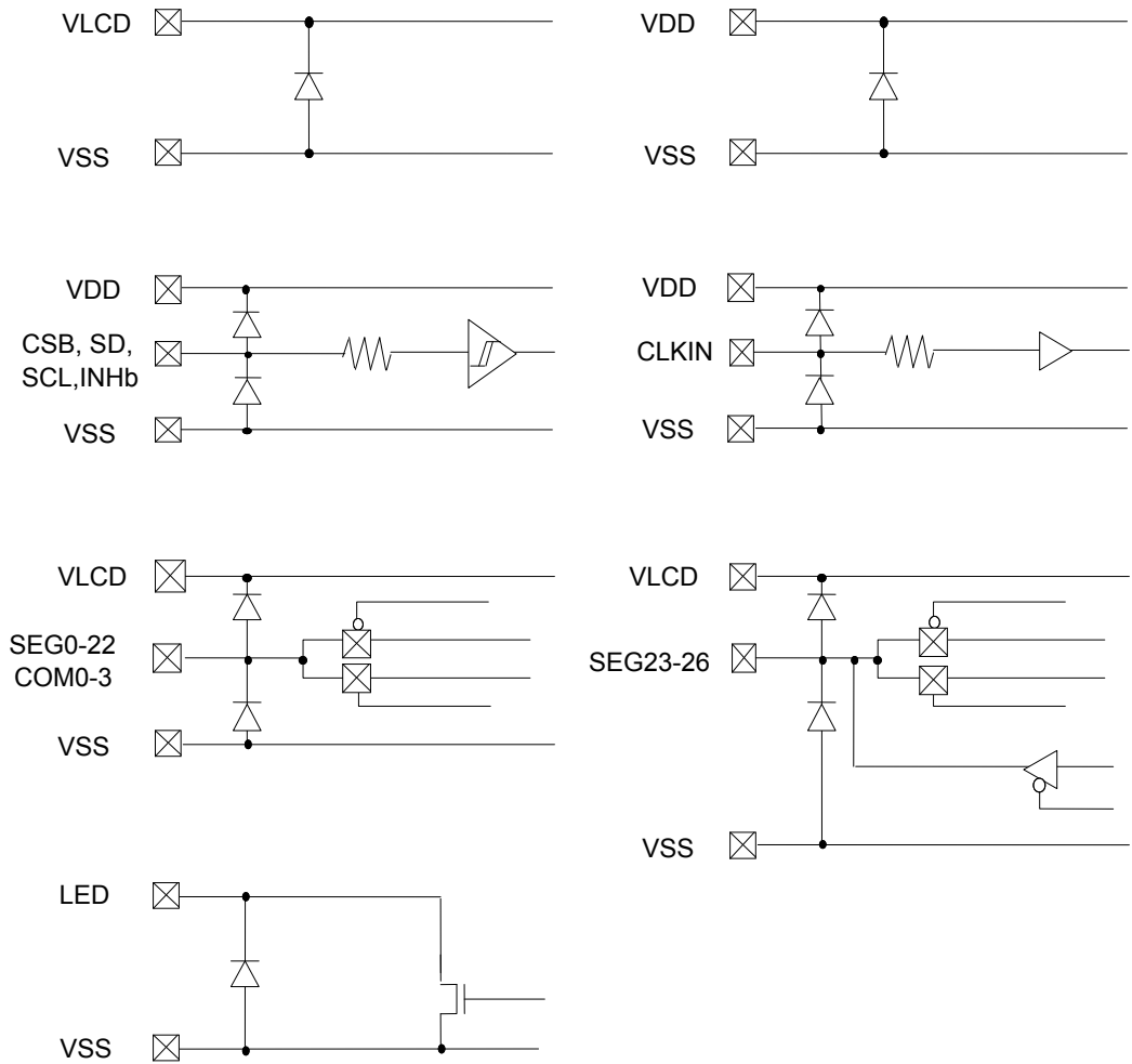
Fig.15 I/O equivalent circuit
