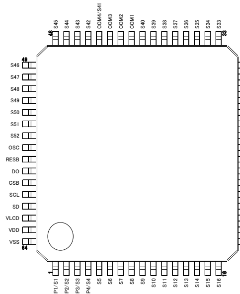
Fig.14 Pin Arrangement (BU97500KV)
