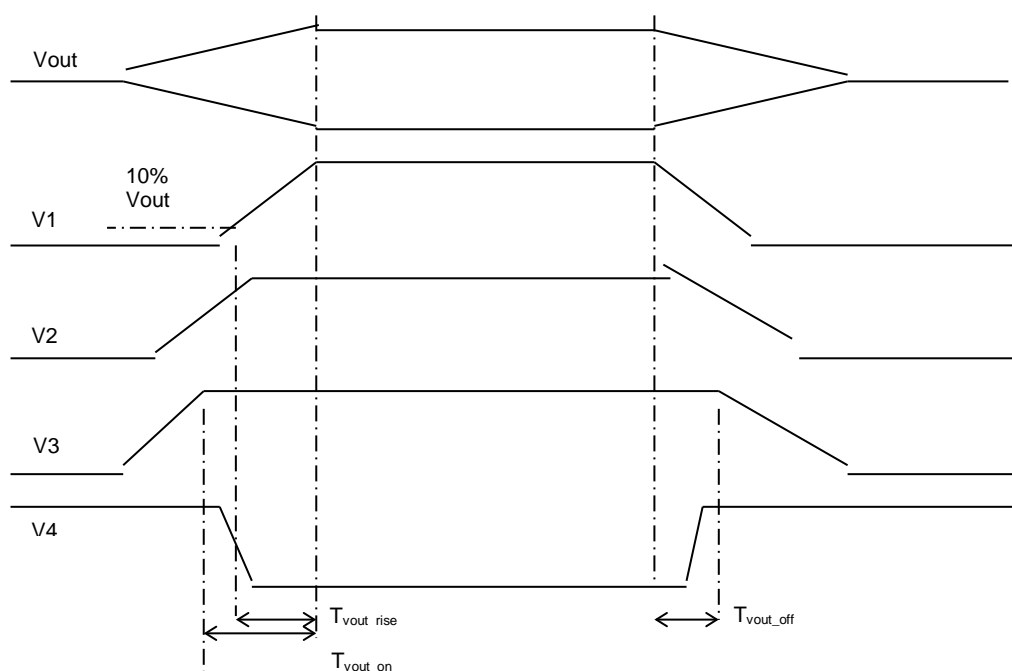
Figure 30. Output Voltage Timing
