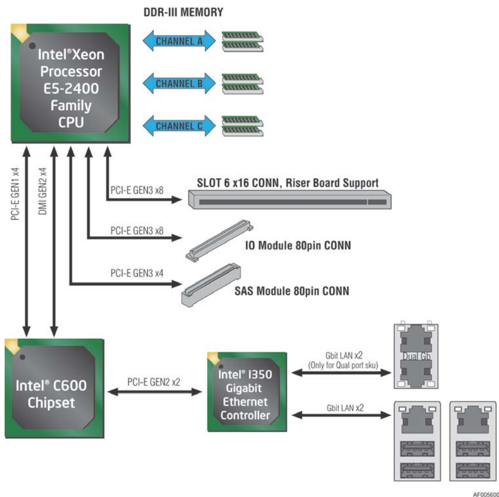
Figure 17. Functional Block Diagram of Processor IIO Sub-system
