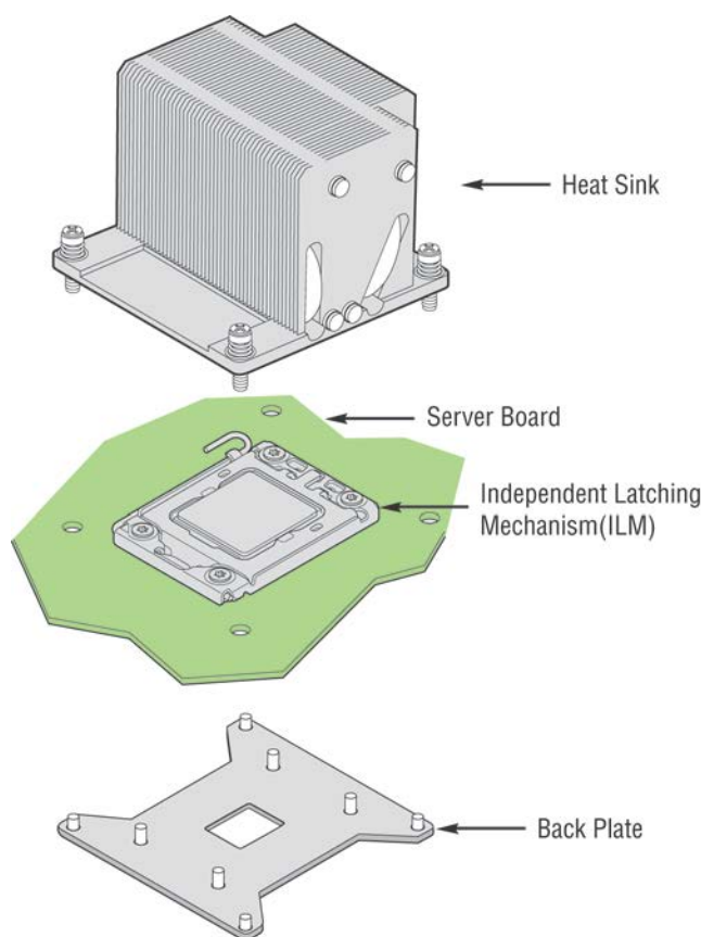
Figure 15. Processor Socket Assembly
