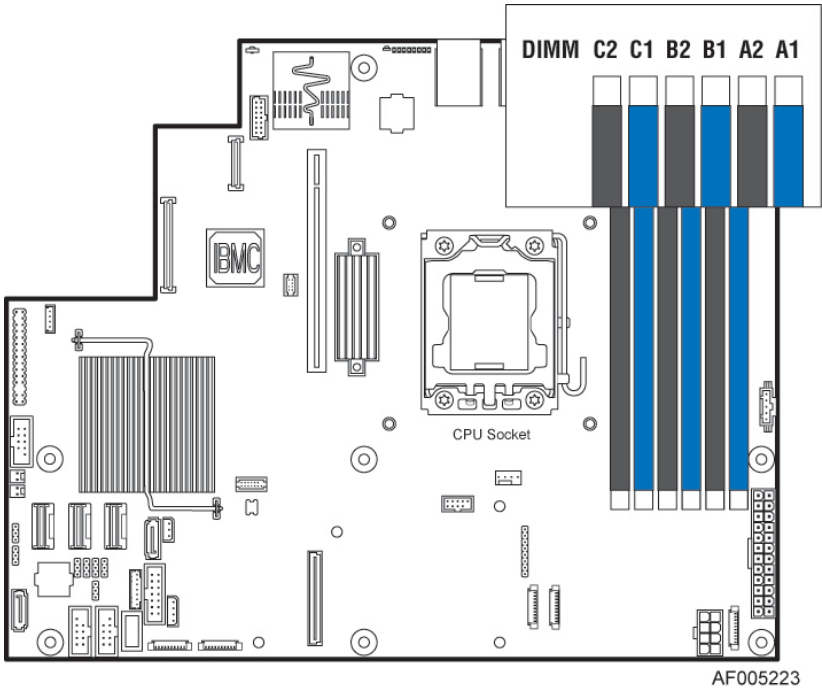
Figure 16. Intel® Server Board S1400SP DIMM Slot Layout
