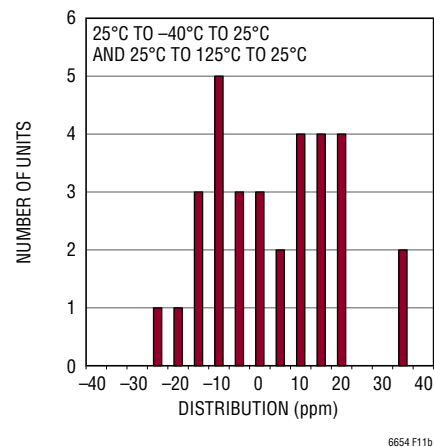
Figure 11b. LT6654 LS8 Thermal Hysteresis -40°C to 125°C
