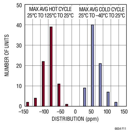
Figure 11a. LT6654 S6 Thermal Hysteresis -40°C to 125°C
