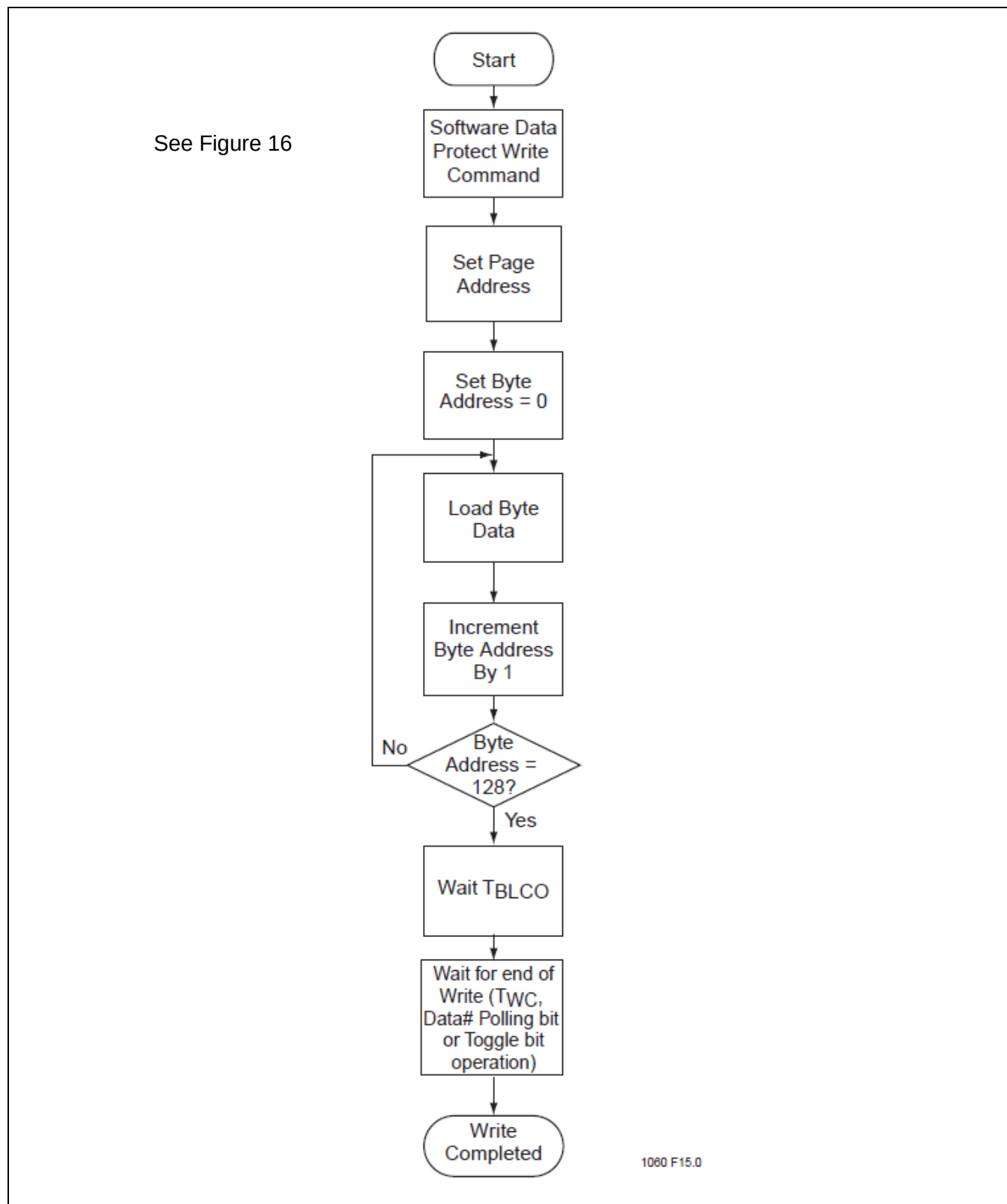
Figure 14: Write Algorithm
