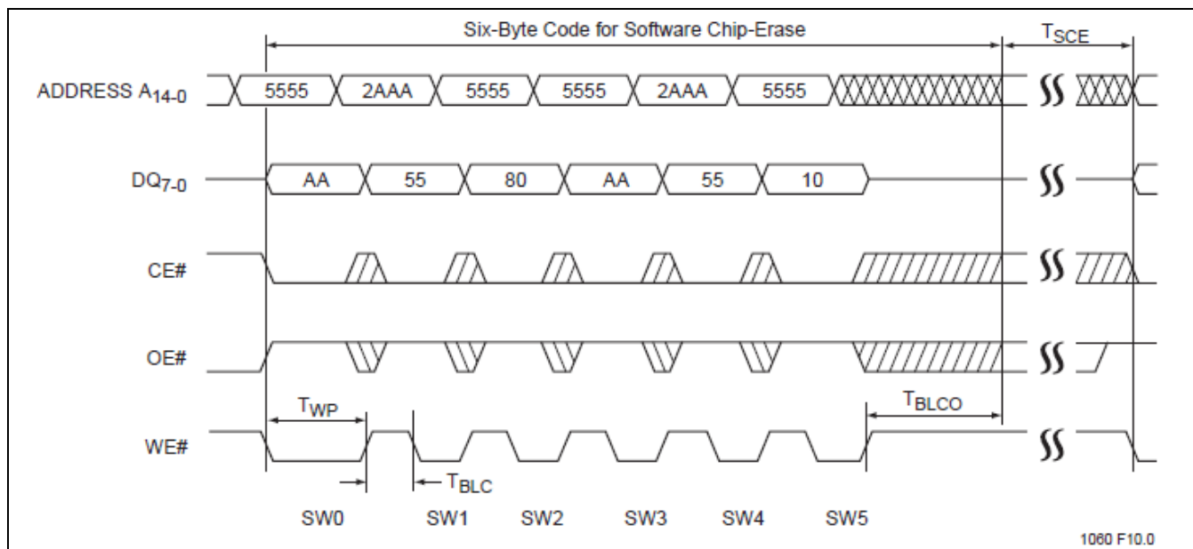
Figure 9: Software Chip-Erase Timing Diagram
