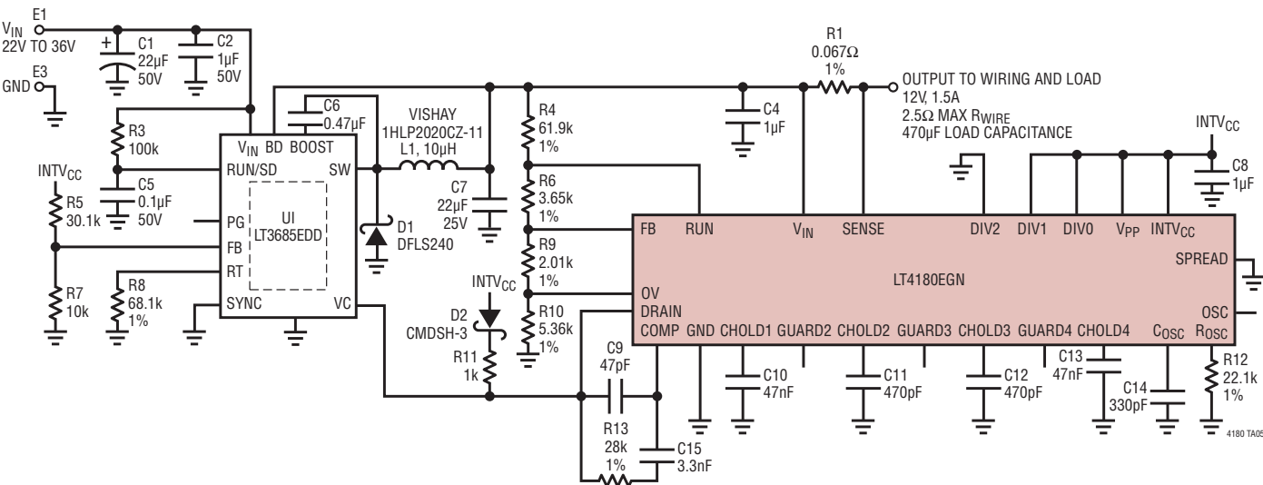
12V 1.5A Buck Regulator
