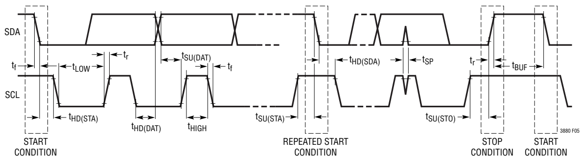
Figure 5. Timing Diagram
