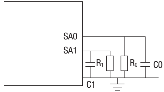
Figure 1. Schematic of Connection of Address Resistors
