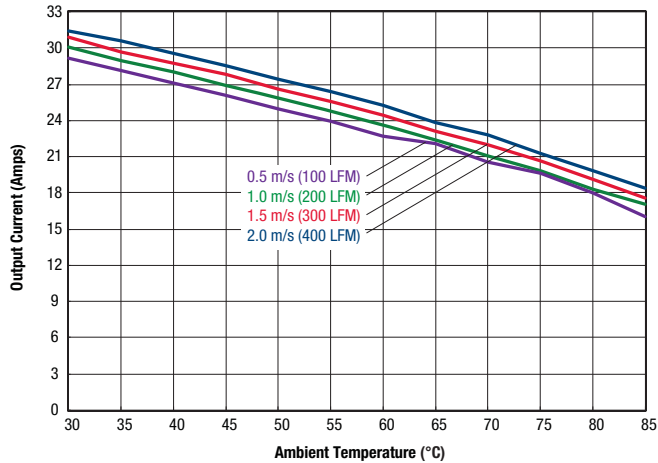
Open Frame
