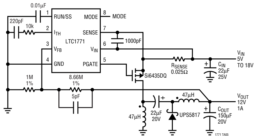
12V/1A Zeta Converter
