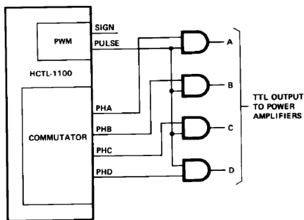
Figure 9. PWM Interface to Brushles DC Motors.
