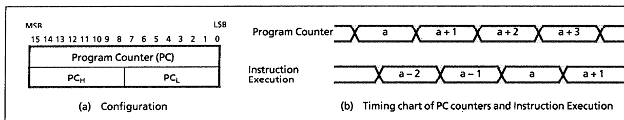
Figure 1-3. Program counter
