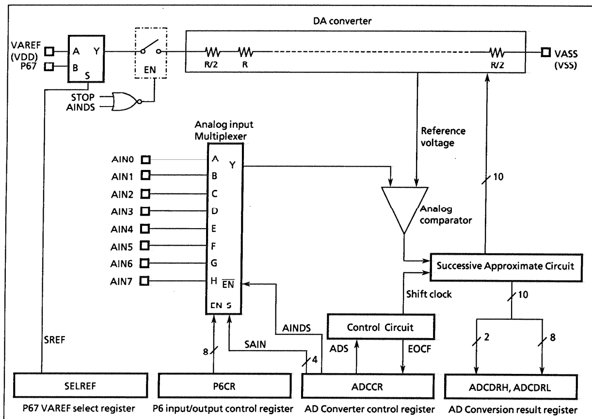
Figure 2-51. AD Converter
