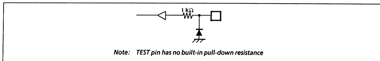
Figure 1-2. TEST Pin
