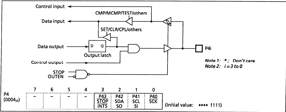
Figure 2-4. Port P4
