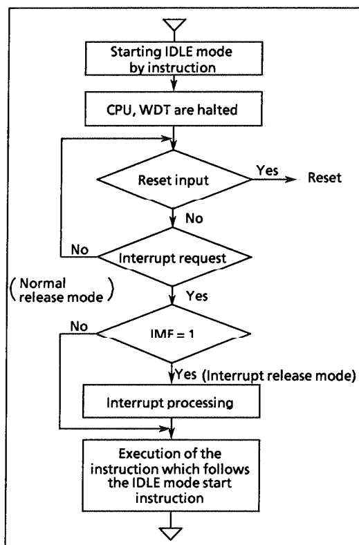
Figure 1-18. IDLE mode
