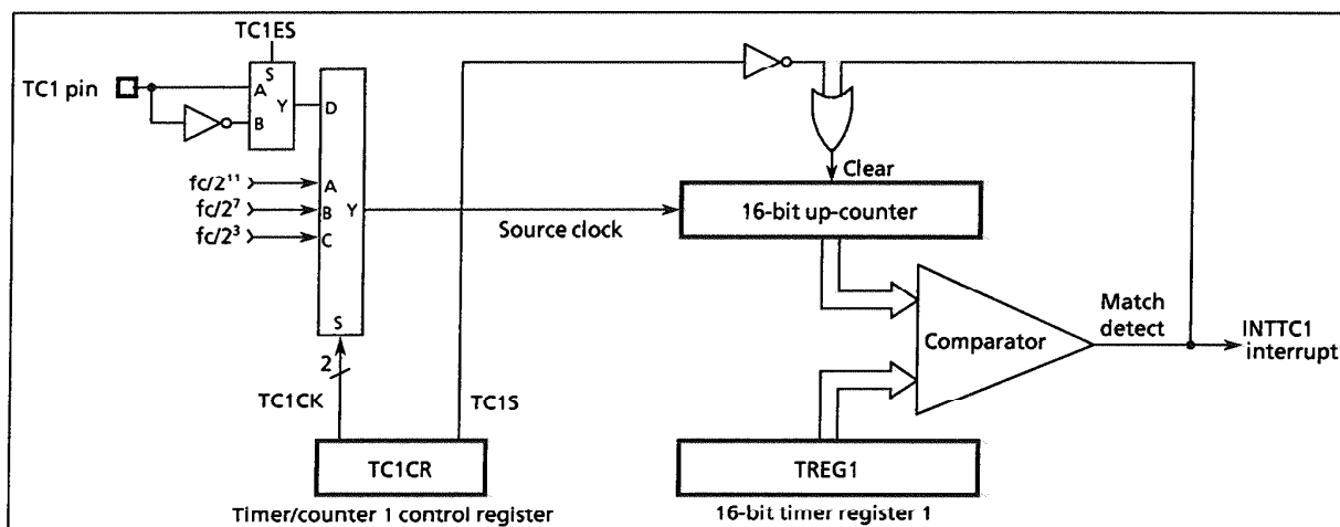
Figure 2-11. Timer/Counter 1
