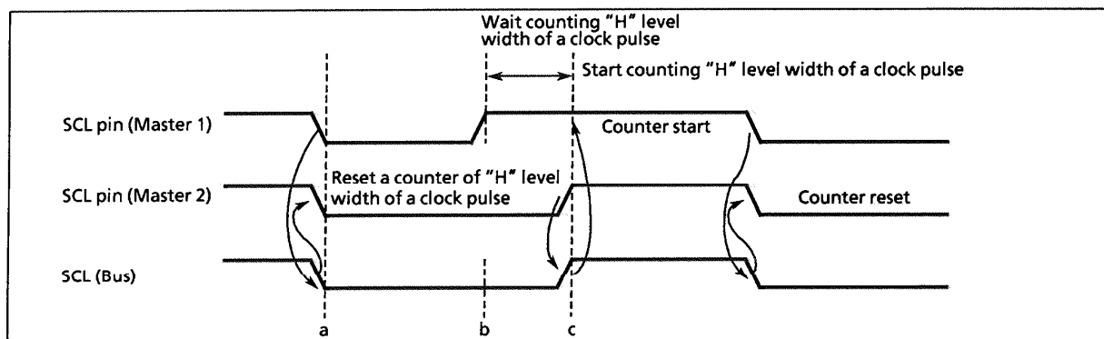
Figure 2-27. Clock synchronization
