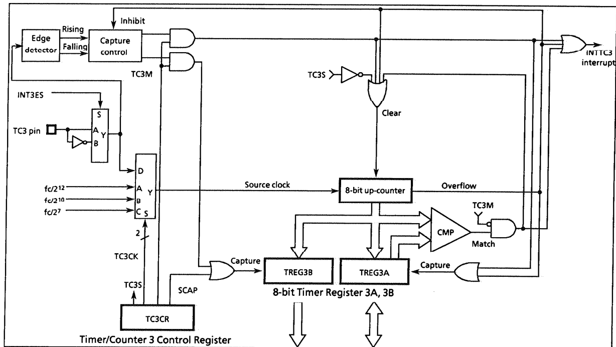
Figure 2-15. Timer/Counter 3
