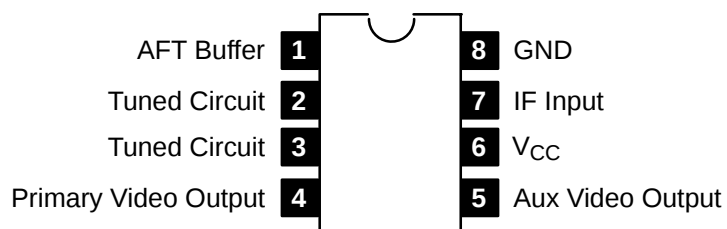
Pin Connection Diagram
