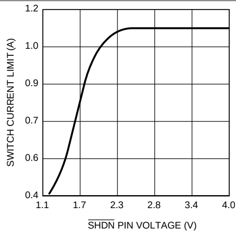
Figure 7. Switch Current Limit vs SHDN Pin Voltage
