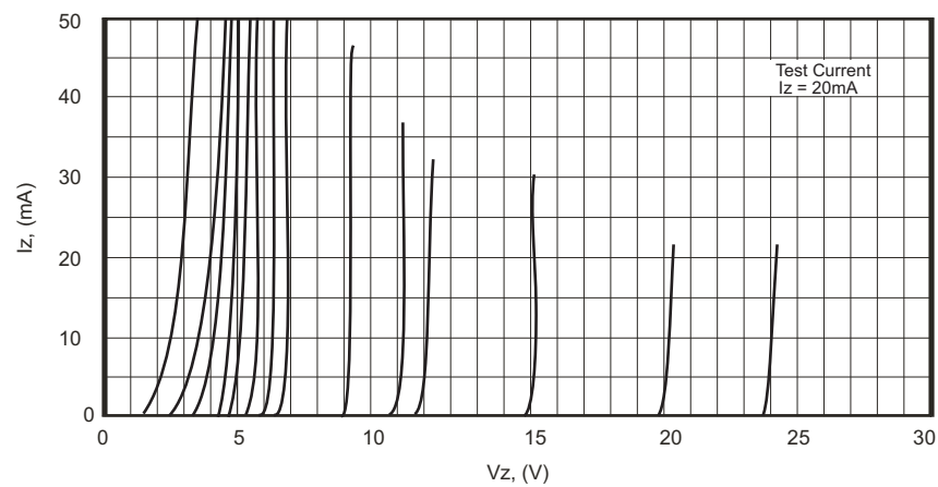
Fig.2 - Breakdown Characteristics
