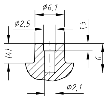
Detail "X" M 2:1
