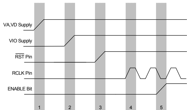
Figure 9. Initialization Sequence
