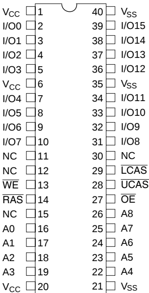
(Top view)
