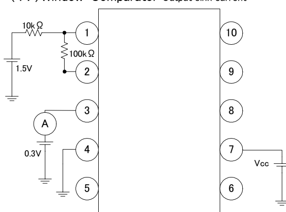
(17) Window-Comparator Output sink current
