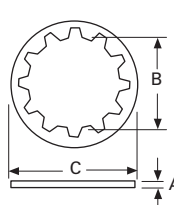
Internal Tooth Lockwasher
