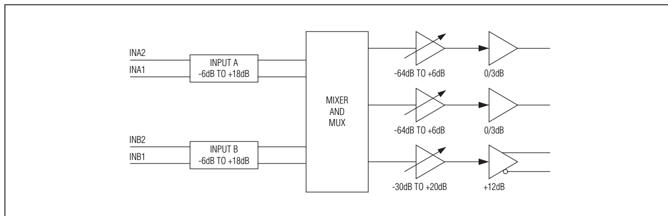
Figure 2. Signal Path
