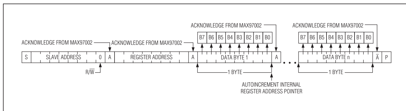
Figure 11. Writing n-Bytes of Data to the MAX97002
