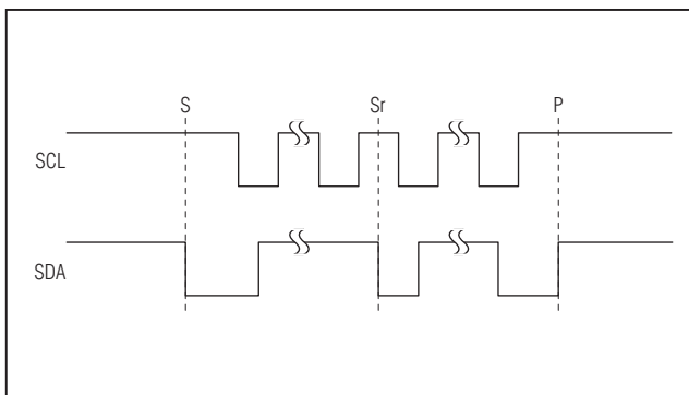
Figure 8. START, STOP, and REPEATED START Conditions
