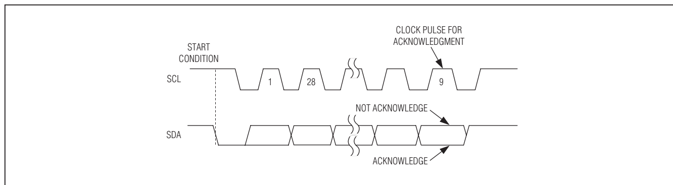
Figure 1. I 2 C Interface Timing Diagram
