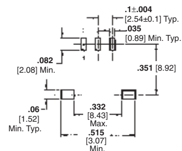
Recommended P.C.B. Pad Layout
