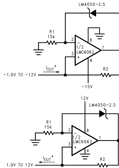
Figure 16. Precision 1-μA to 1-mA Current Source (±)
