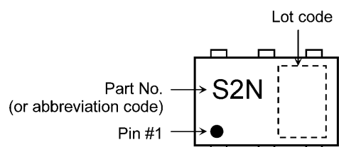
Fig. 7.1 Marking
