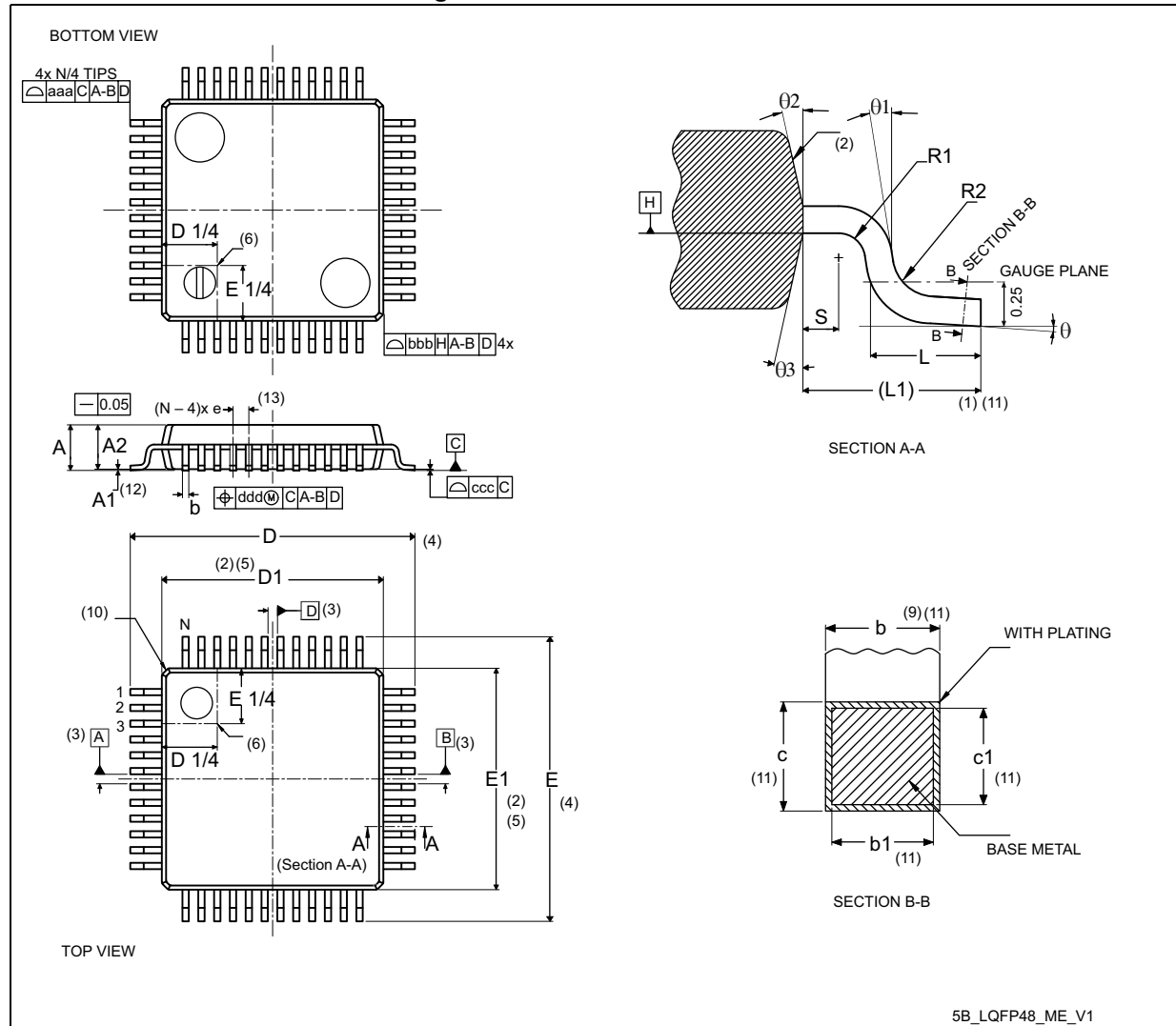
Figure 57. LQFP48 - Outline (15)
