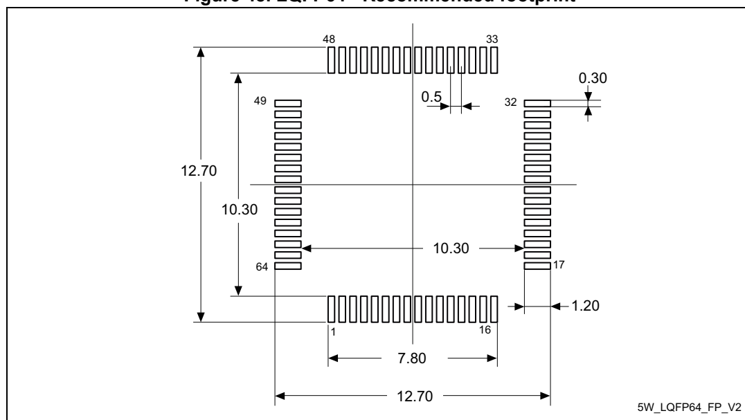
Figure 48. LQFP64 - Recommended footprint
