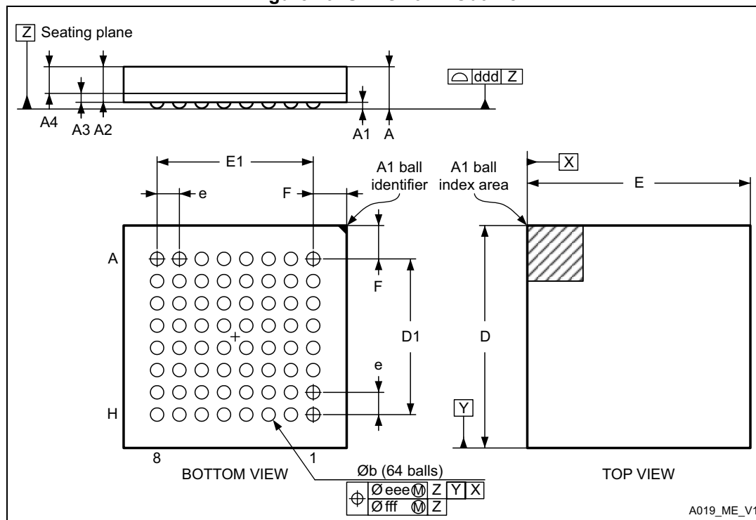
Figure 49. UFBGA64 – Outline
