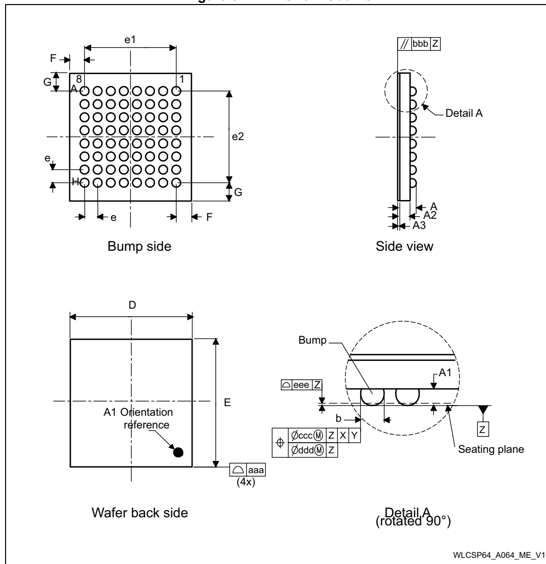
Figure 51. WLCSP64 -Outline
