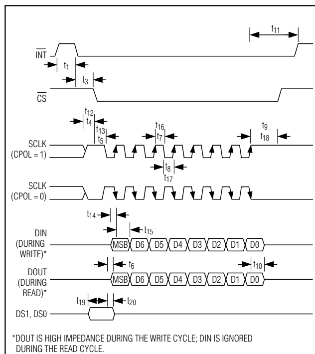
Figure 4. Serial-Interface Timing
