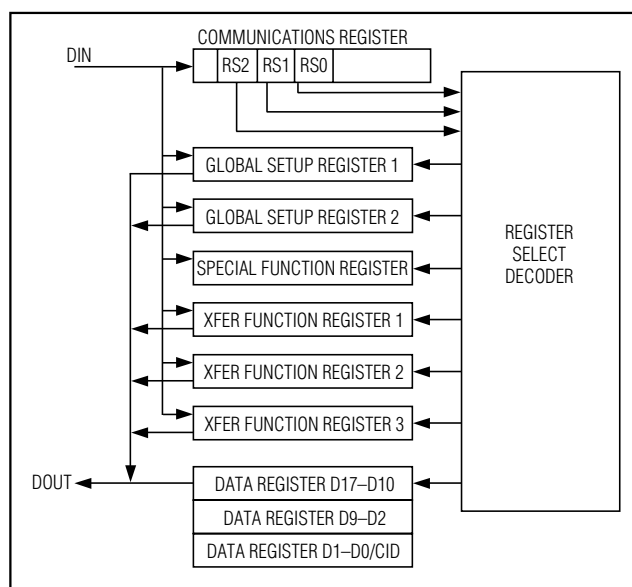
Figure 3. Register Summary
