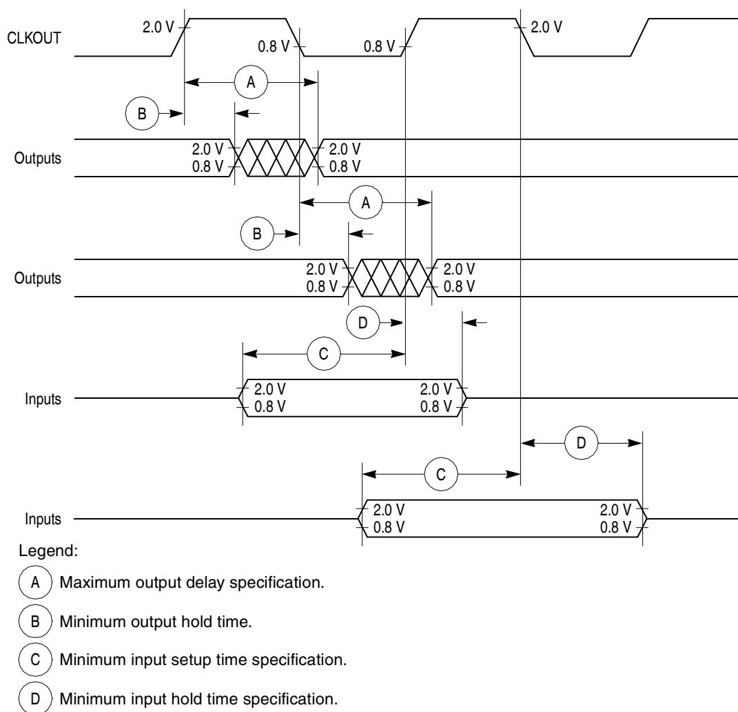
Figure 4. Control Timing
