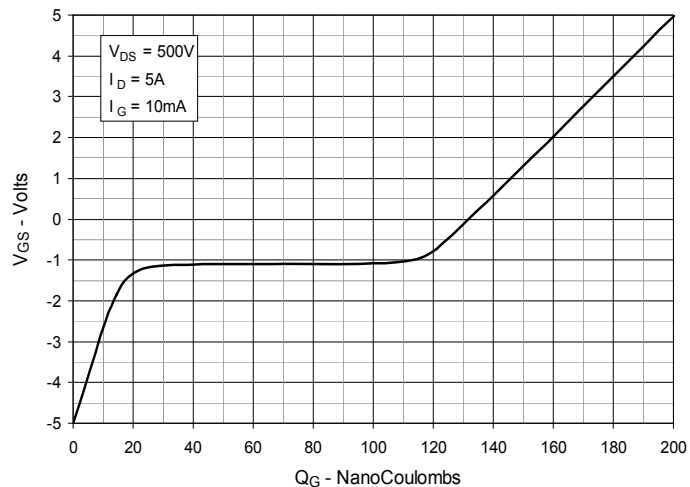
Fig. 14. Gate Charge
