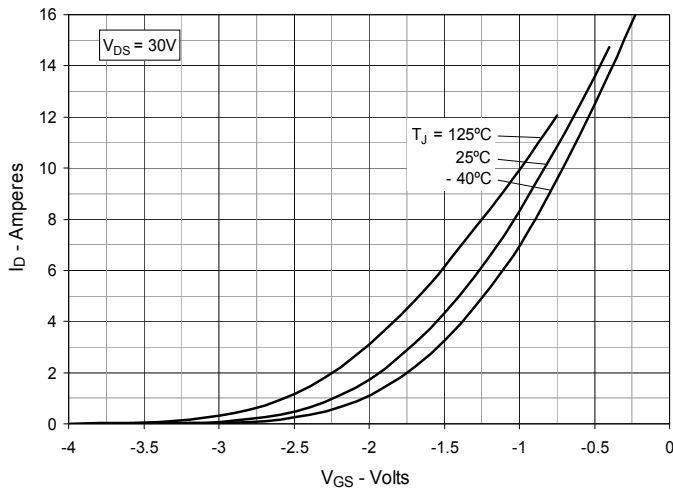
Fig. 9. Input Admittance
