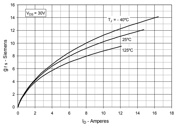
Fig. 10. Transconductance
