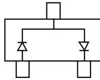
BAS70H-04 Marking: K74
