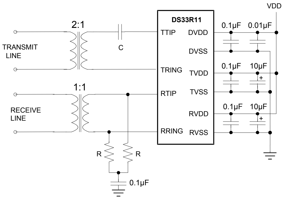
Figure 10-7. Basic Interface
