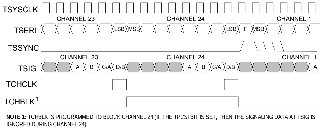
Figure 12-18. Transmit-Side 1.544MHz Boundary Timing (Elastic Store Enabled)
