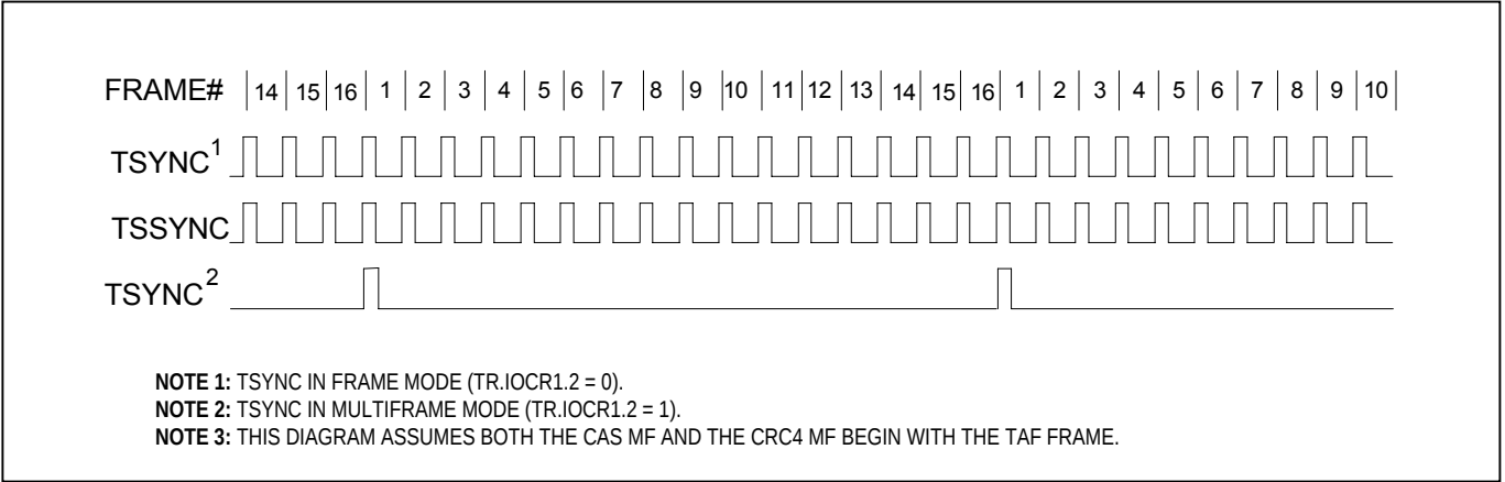
Figure 12-25. Transmit-Side Timing
