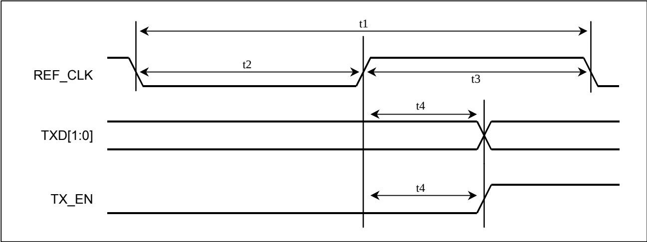
Figure 13-3. Transmit RMII Interface Timing
