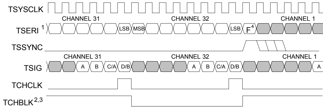
Figure 12-19. Transmit-Side 2.048MHz Boundary Timing (Elastic Store Enabled)
