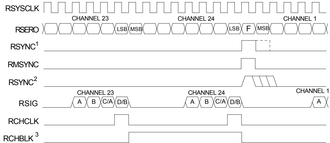
Figure 12-13. Receive-Side 1.544MHz Boundary Timing (Elastic Store Enabled)
