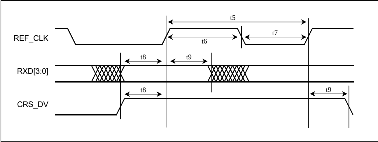
Figure 13-4. Receive RMII Interface Timing
