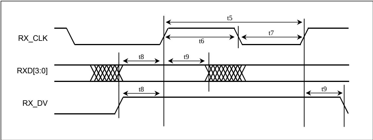
Figure 13-2. Receive MII Interface Timing
