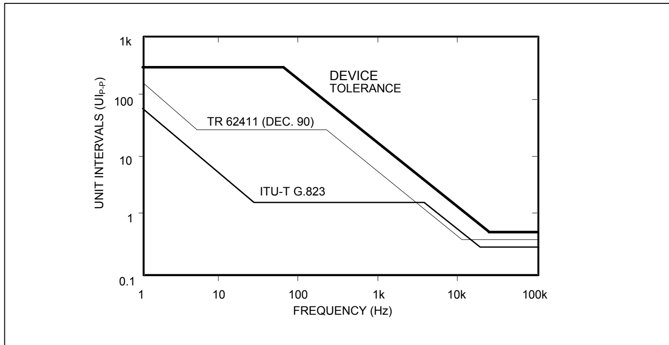
Figure 10-10. Jitter Tolerance
