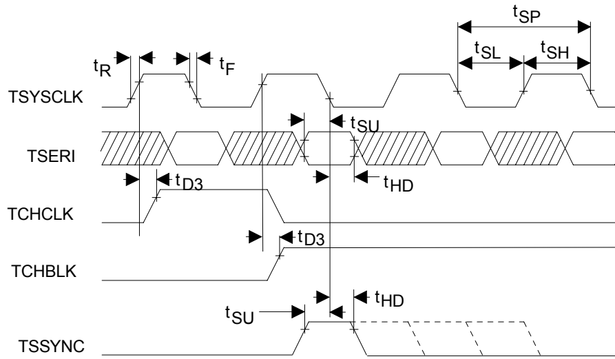
Figure 13-18. Transmit-Side Timing, Elastic Store Enabled
