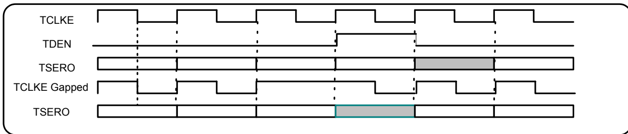
Figure 12-1. Tx Serial Interface Functional Timing
