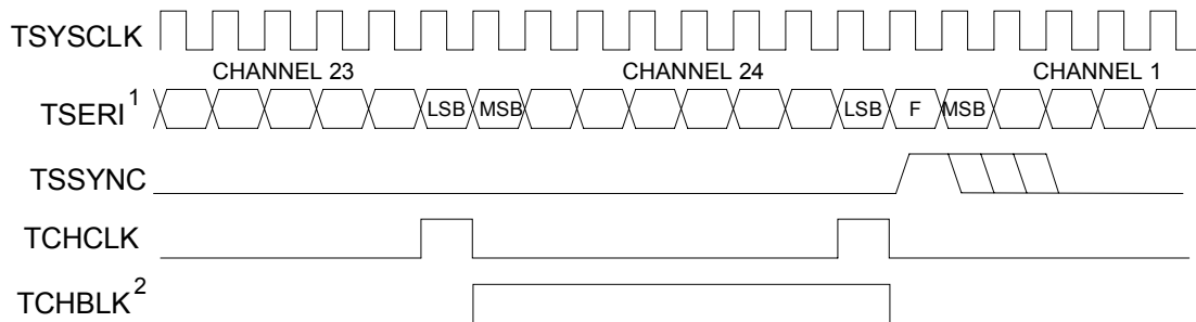
Figure 12-27. Transmit-Side Boundary Timing, TSYSCLK = 1.544MHz (Elastic Store Enabled)
