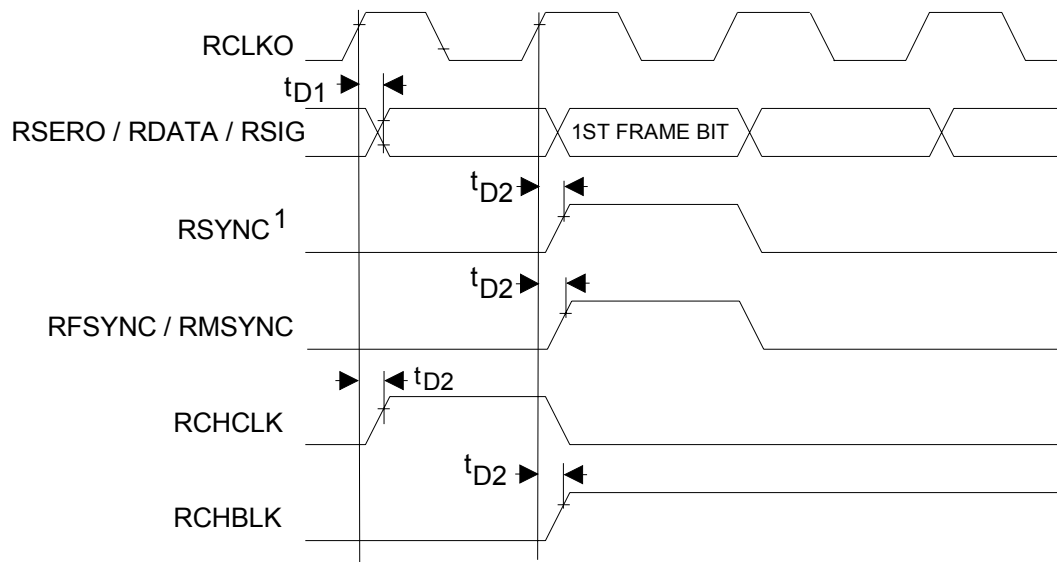
Figure 13-13. Receive-Side Timing
