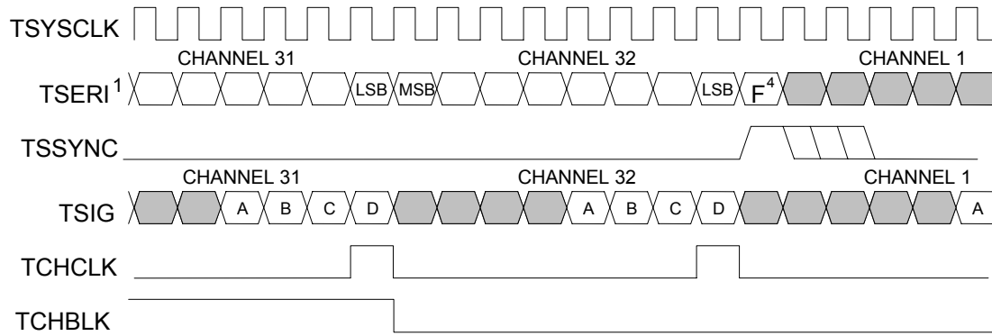
Figure 12-28. Transmit-Side Boundary Timing, TSYSClk = 2.048MHz (Elastic Store Enabled)
