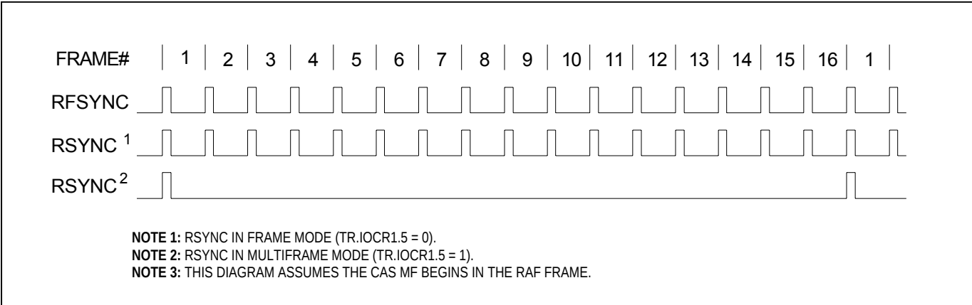
Figure 12-20. Receive-Side Timing
