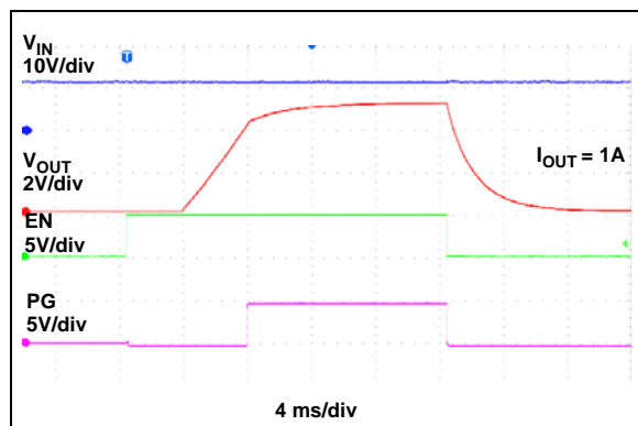
FIGURE 2-31: Enable Turn-On and Turn-Off.
