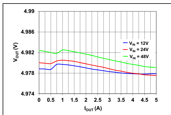
FIGURE 2-8: Output Voltage vs. Output Current ( V_{OUT} = 5V ).
