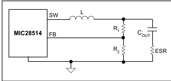
FIGURE 5-2: Enough Ripple at FB.
