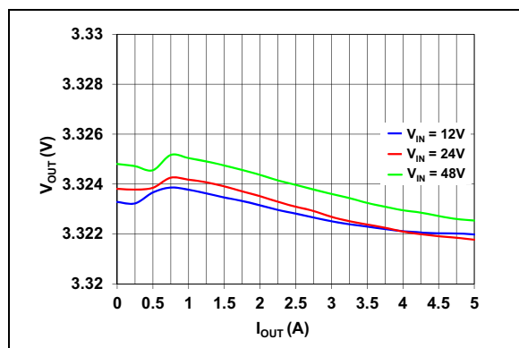
FIGURE 2-7: Output Voltage vs. Output Current ( V_{OUT} = 3.3V ).
