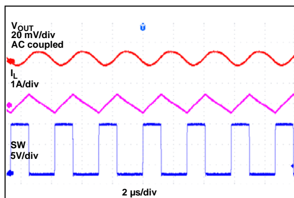
FIGURE 2-32: Switching Waveform ( I_{OUT} = 0A ).
