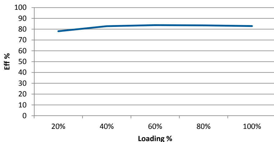
AM2D-0505SZ Efficiency vs. Loading
