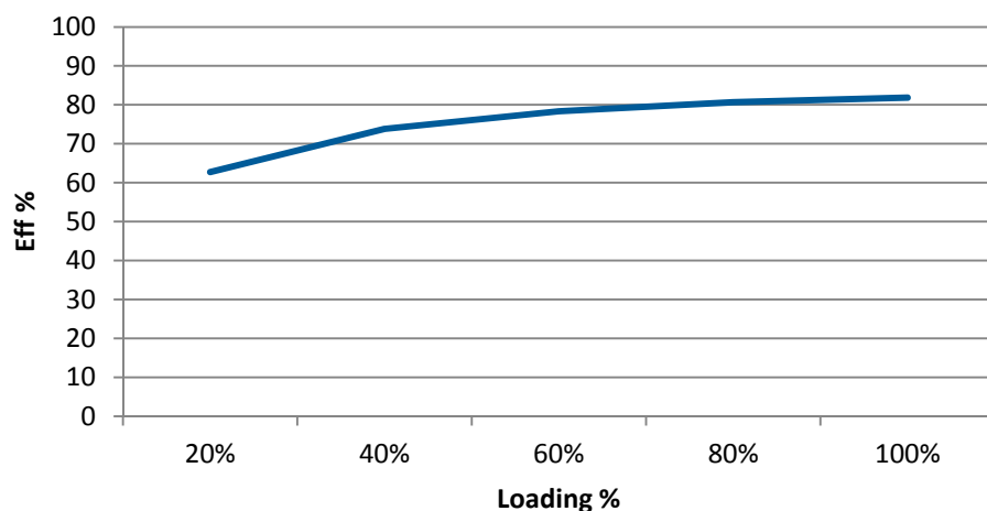
AM2D-1205SZ Efficiency vs. Loading
