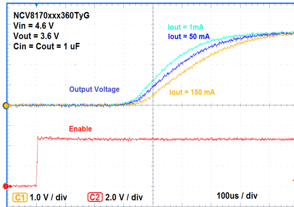
Figure 43. Enable Turn-on Response at V_{out} = 3.6\text{ V}
