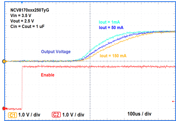
Figure 42. Enable Turn-on Response at V_{out} = 2.5\text{ V}
