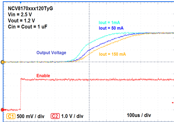
Figure 41. Enable Turn-on Response at V_{out} = 1.2\text{ V}
