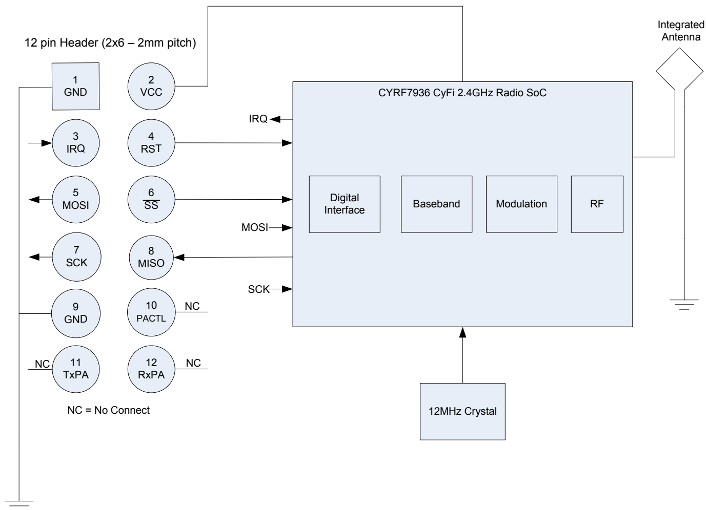
Figure 1 - Module Schematic
