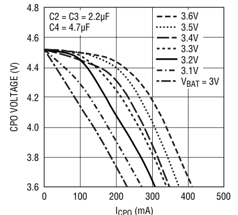
1.5x Mode CPO Voltage vs I_{CPO}
