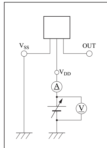
Figure 5-b Measurement Circuit
