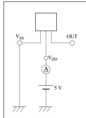
Figure 6-b Measurement Circuit
