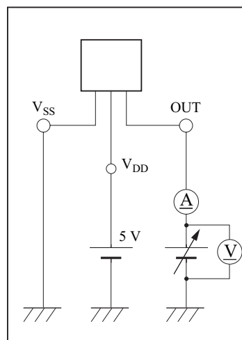
Figure 12-b Measurement Circuit
