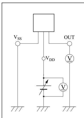
Figure 8-b Measurement Circuit
