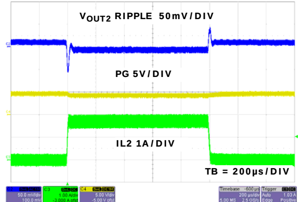
FIGURE 21. LOAD TRANSIENT CHANNEL 2 (PWM)
