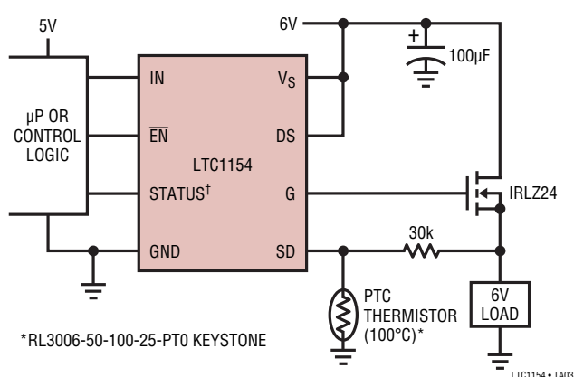
High Side Driver with Thermal Shutdown
